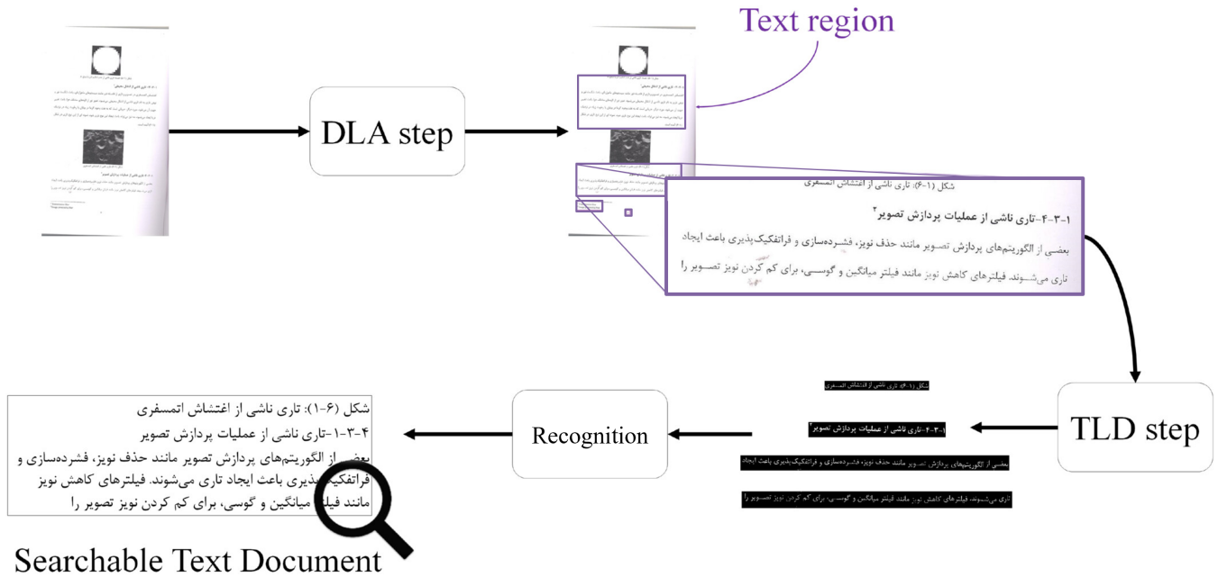
Figure 1: Stages of OCR pictured on a Persian Document: Document Layout Analysis, Text Line Detection, and Recognition. Modified from Fateh et al. [4].
